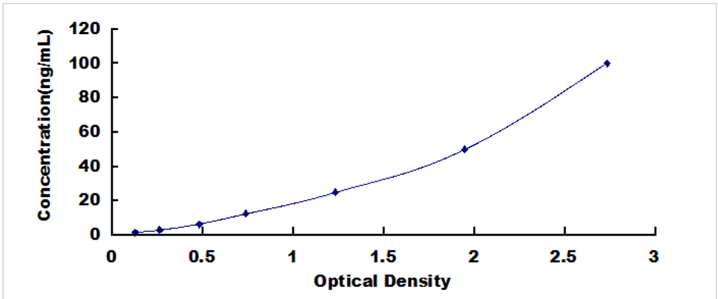
Typical Standard Curve for LDHD, Human ELISA.
