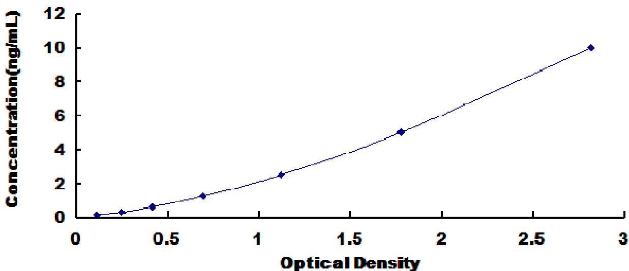
Typical Standard Curve for KLF5, Human ELISA.
