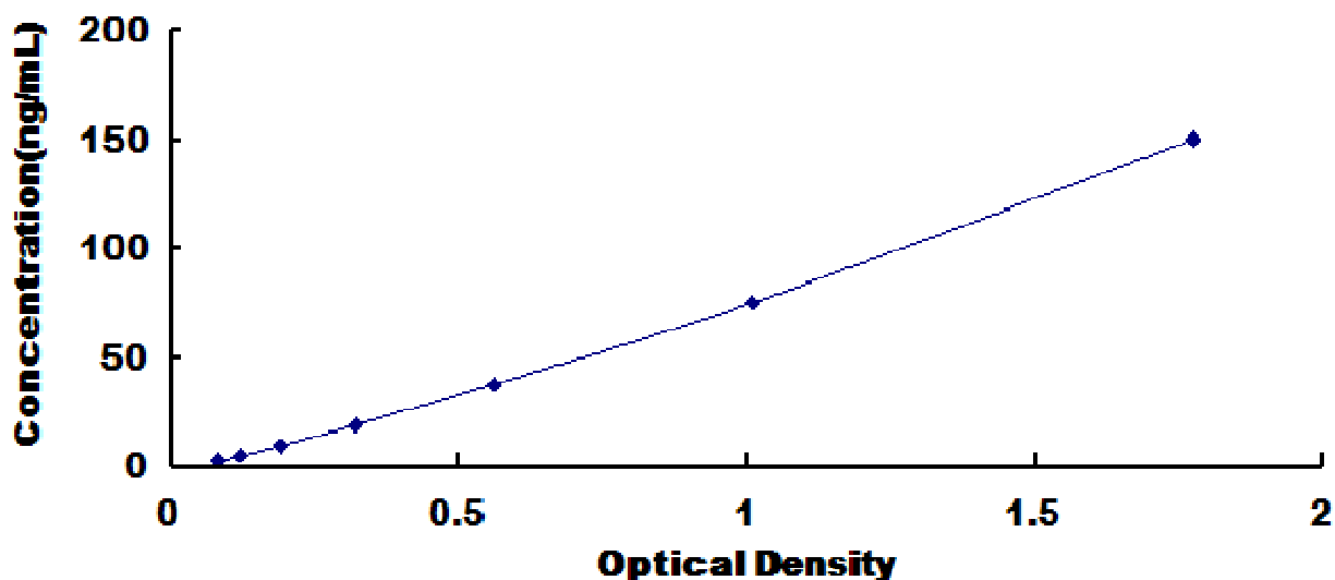
Typical Standard Curve for HDC, Human ELISA.
