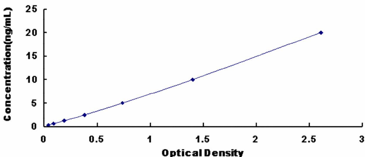
Typical Standard Curve for HRH3, Rat ELISA.
