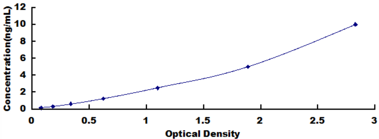
Typical Standard Curve for GSTa3, Human ELISA.
