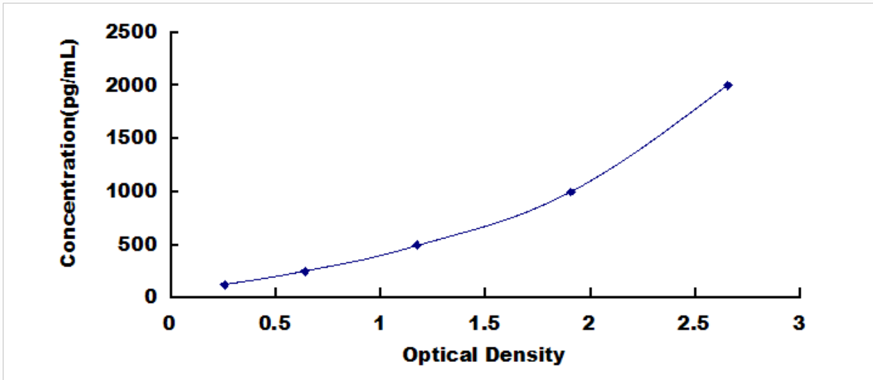
Typical Standard Curve for FcgR3A, Human ELISA.
