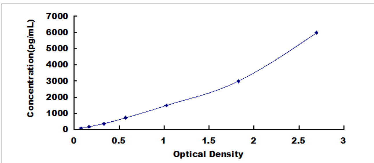
Typical Standard Curve for ENPP2, Human ELISA.
