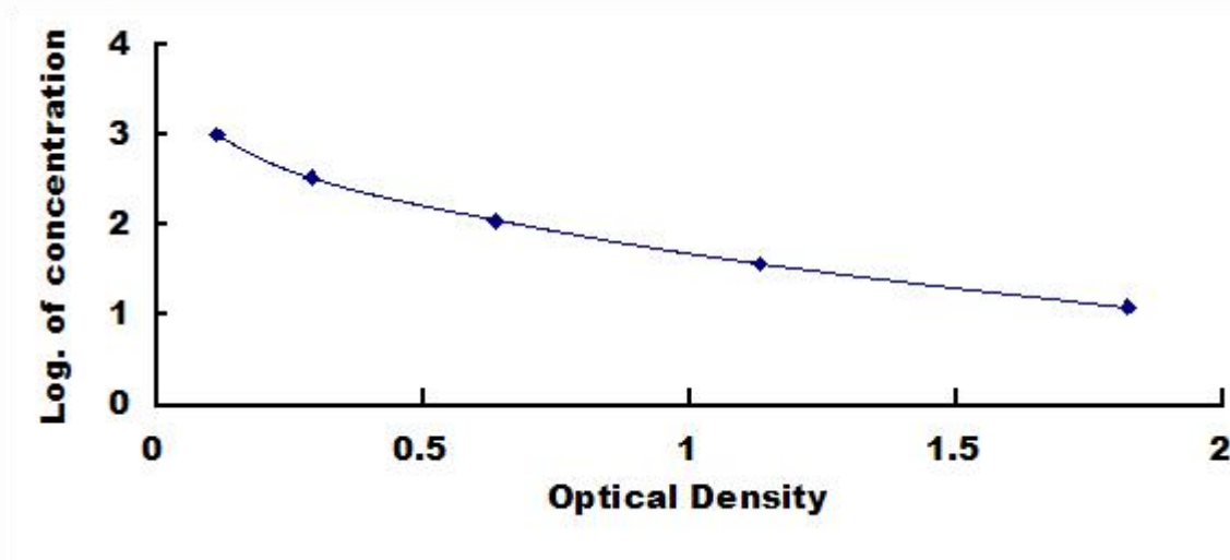
Typical Standard Curve for Deoxycholate ELISA.
