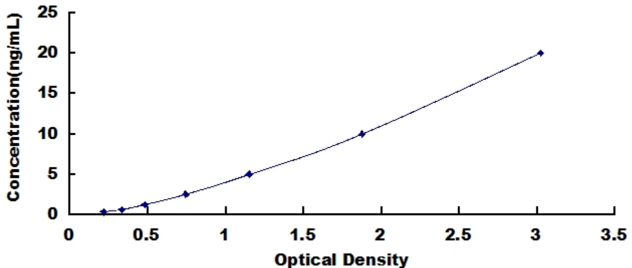
Typical Standard Curve for CYP1A1, Rat ELISA.
