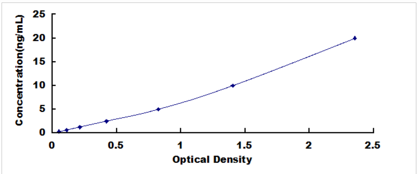
Typical Standard Curve for CLIC4, Rat ELISA.
