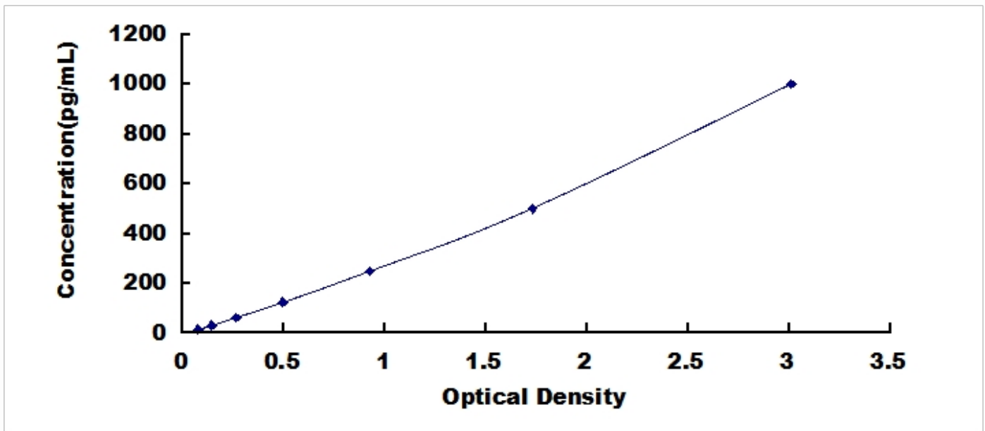
Typical Standard Curve for ANGPTL8, Mouse ELISA.
