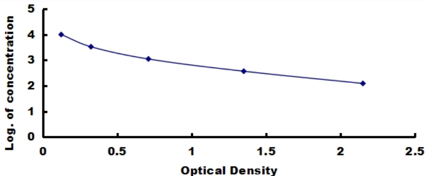
Typical Standard Curve of ELISA Assay for T3.
