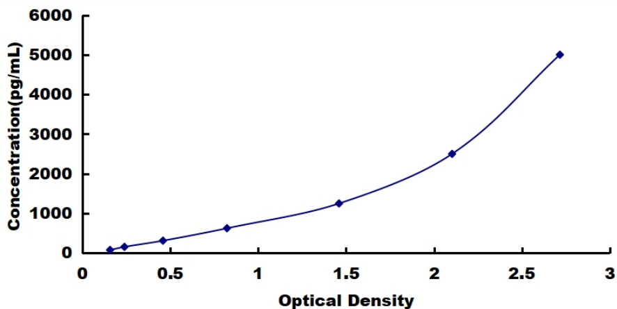
Typical Standard Curve of ELISA Assay for Human, RNASE3.
