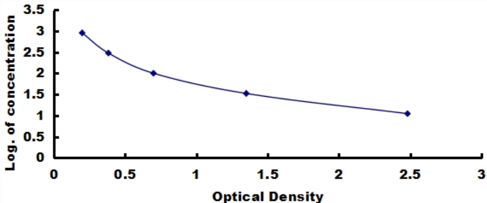
Typical Standard Curve of ELISA Assay for 5-HT.
