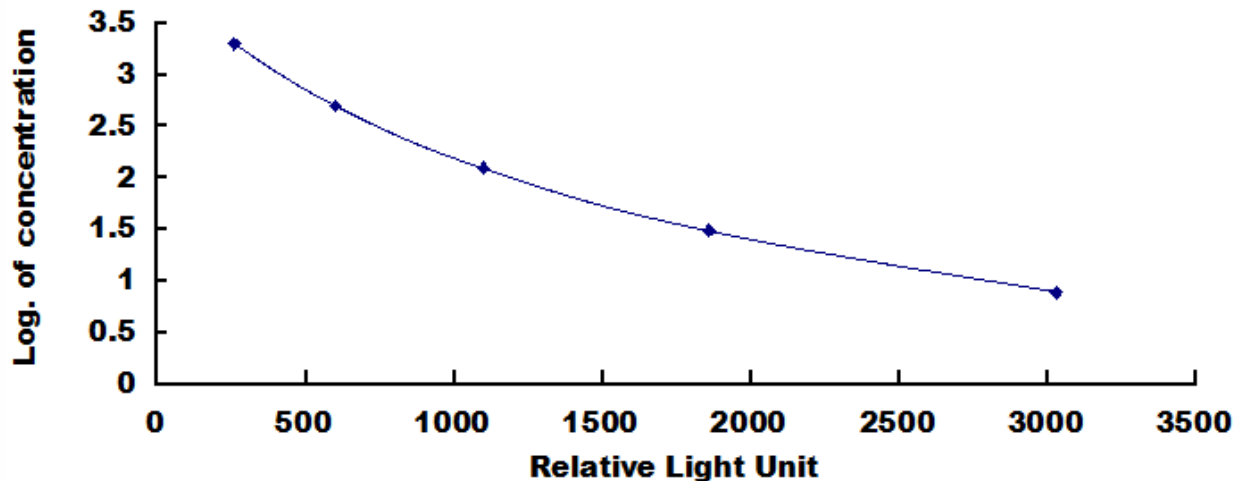
Typical Standard Curve for PTH, Rat CLIA.
