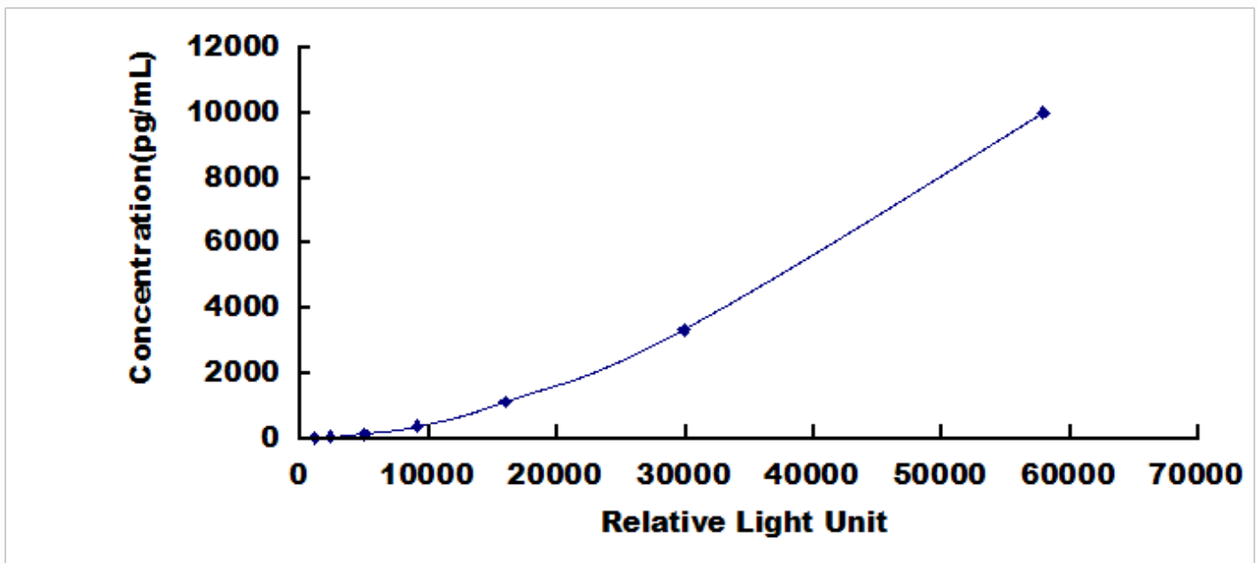
Typical Standard Curve for MMP7, Human CLIA.
