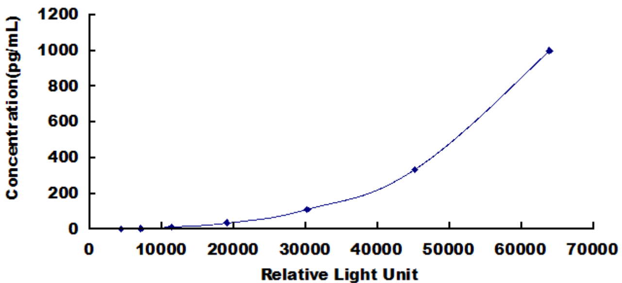
Typical Standard Curve for IL21, Human CLIA.
