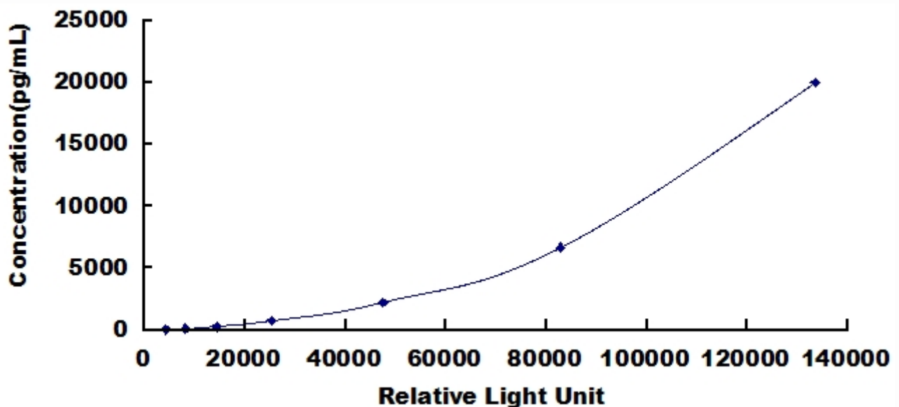
Typical Standard Curve for IGF1, Bovine CLIA.
