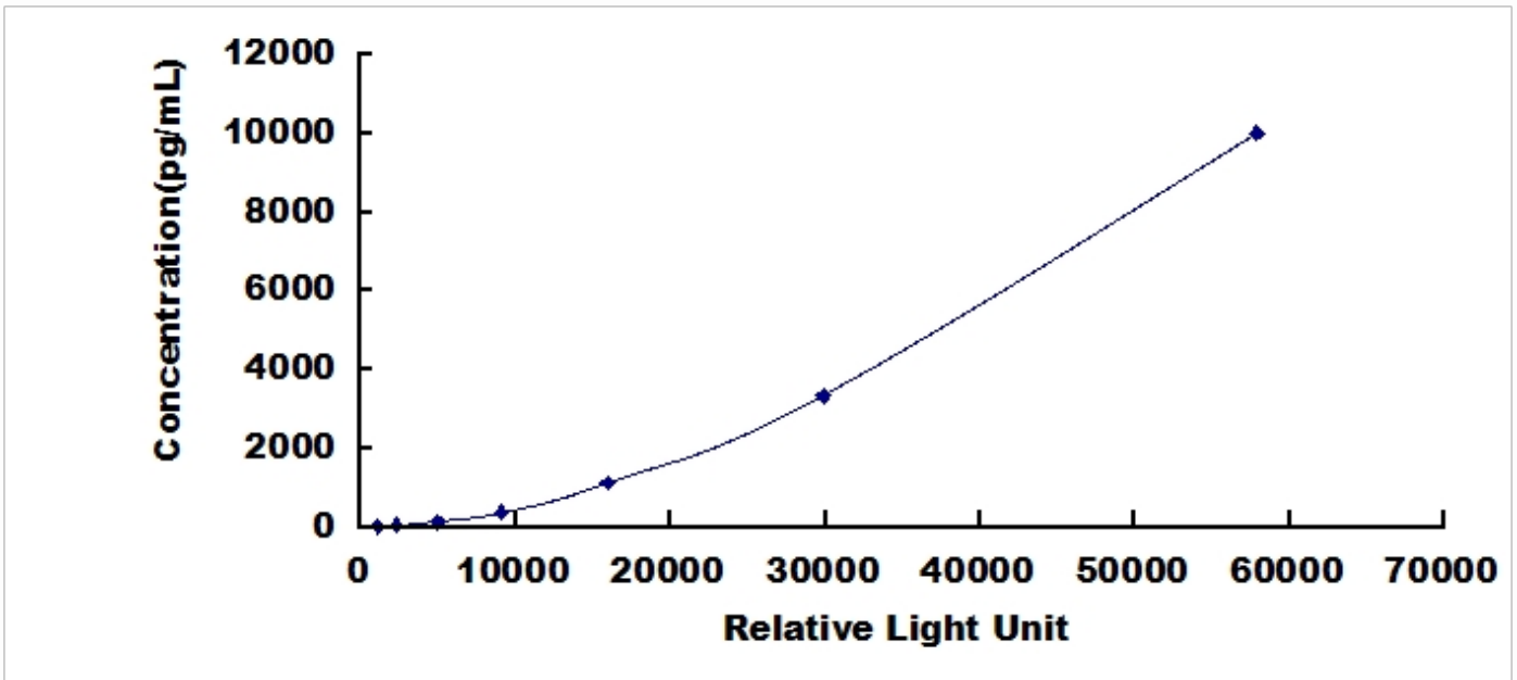
Typical Standard Curve for IgE, Porcine CLIA.
