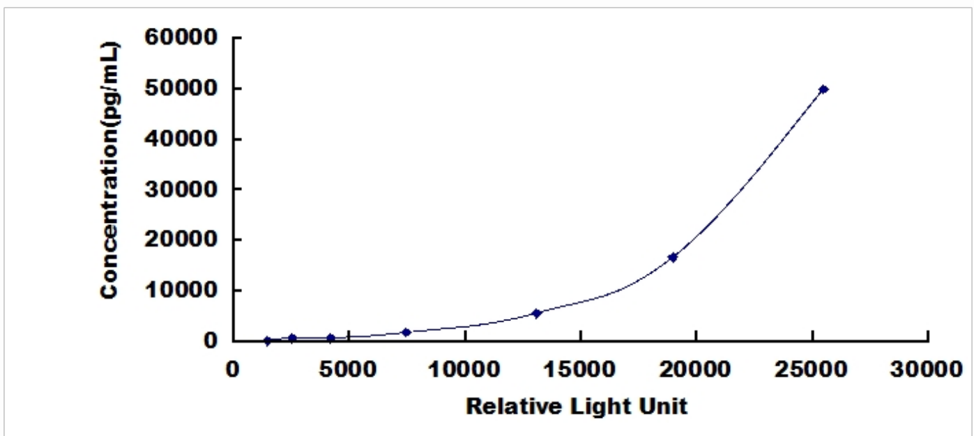
Typical Standard Curve for GAL1, Human CLIA.
