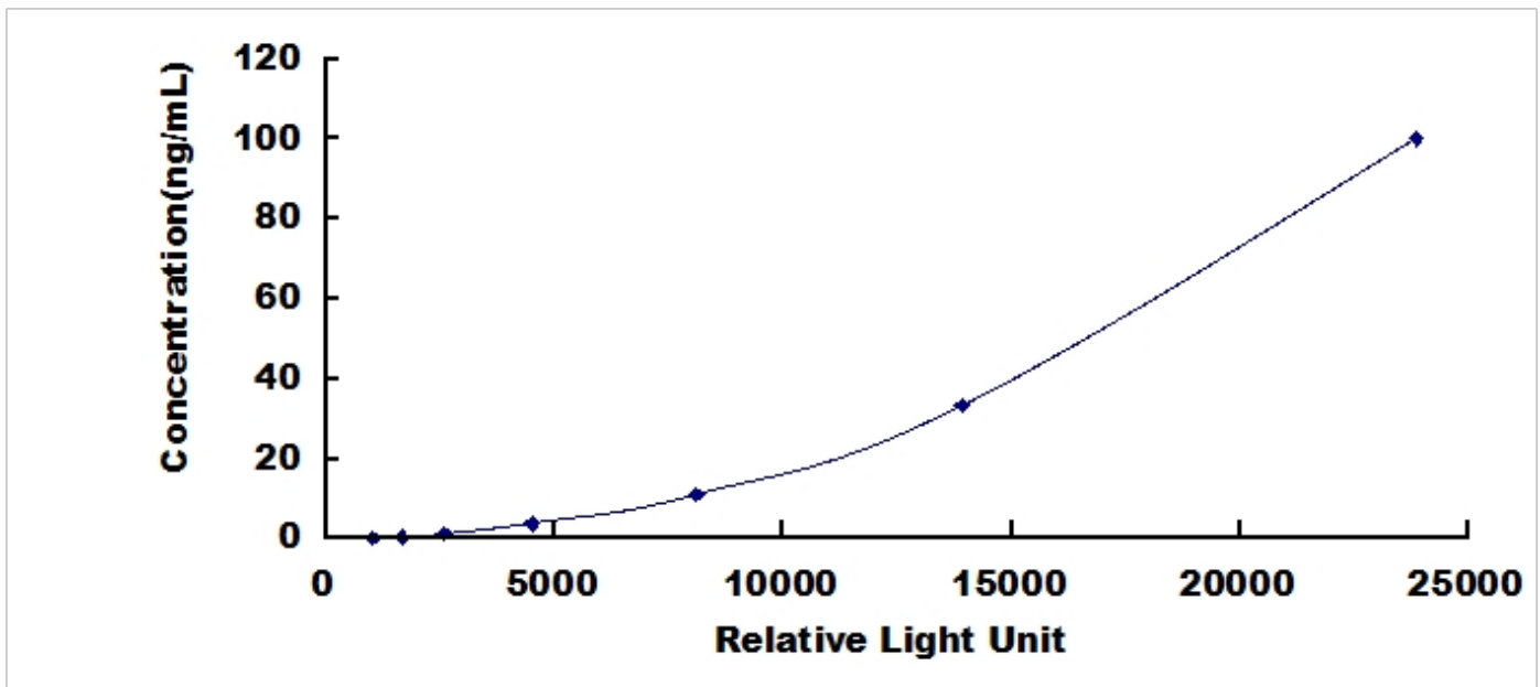
Typical Standard Curve for C1INH, Human CLIA.
