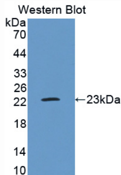
Used in Western Blot, Sample: Recombinant Ki67P, Human
