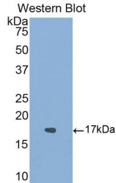
Used in Western Blot, Sample: Recombinant ACVR1, Human
