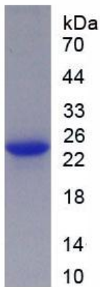
Figure 4. SDS-PAGE
